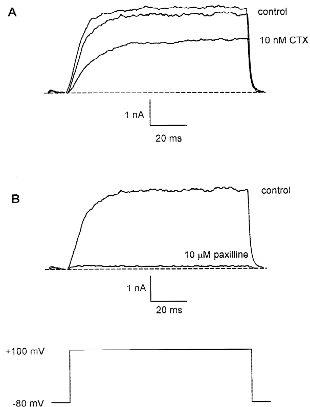
Fig. 5. Effects of CTX and paxilline on the steady state current in C1 cells with 10 \mu\text{M} [\text{Ca}^{2+}]_i . Currents were elicited by 100 ms steps from a holding potential of -80 \text{ mV} to +100 \text{ mV} every 20 s in \text{Na}^+ solution. Current traces were obtained before, during, and after application of 10 nM CTX (A) to the bath solution or (B) before (control) and 80 s after application of 10 \mu\text{M} paxilline to the bath solution.
