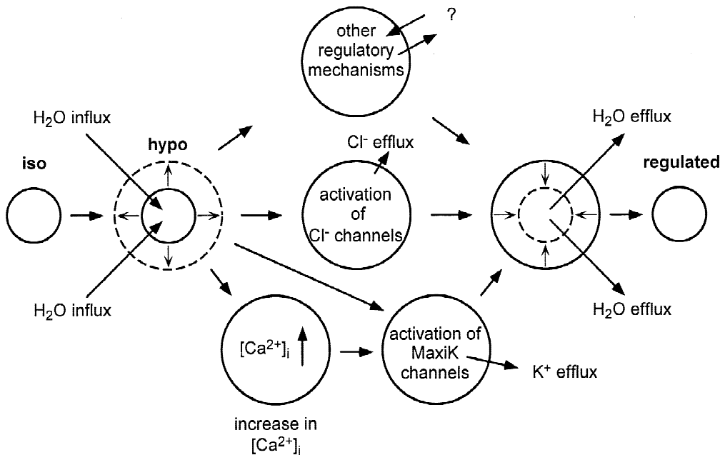
Fig. 8. Proposed model for regulatory volume decrease in osteoblasts.
