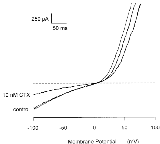
Fig. 6. Membrane currents in C1 cells with 10 \mu\text{M} [\text{Ca}^{2+}]_i . Ramp currents were elicited by voltage ramps from -100 to +100 \text{ mV} within 400 ms at 10 s intervals. Traces were obtained while bathing the cells in a \text{K}^+ solution before, during, and after application of a \text{K}^+ solution containing 10 nM charybdotoxin (CTX).
