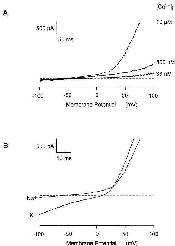
Fig. 3. Effect of [Ca^{2+}]_i on membrane currents in C1 cells. (A) Membrane currents were elicited by voltage ramps from -100 to 100 mV within 400 ms. Current traces shown were measured in different cells in Na^+ solution with pipette solutions that buffer [Ca^{2+}]_i to 33 nM, 500 nM or 10 \mu M. (B) Membrane currents were similarly elicited as described in A (voltage ramps from -100 to 100 mV within 400 ms at 10 s intervals) in either external Na^+ or K^+ solution. The pipette solution was buffered to 10 \mu M [Ca^{2+}]_i .
