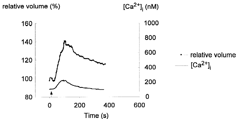
Fig. 2. Changes in [Ca^{2+}]_i and relative volume in C1 cells after application of a hypotonic solution with 500 \mu M EGTA and no added Ca^{2+} . Each curve represents the mean of four cells. The arrow marks the beginning of the solution change. Note the different time scale compared to Fig. 1.
