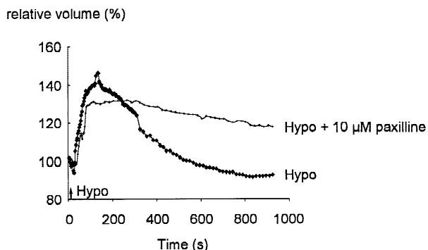
Fig. 7. Changes in relative volume in a single C1 cell after application of a hypotonic solution containing 10 \mu\text{M} paxilline in comparison with volume changes in hypotonic solution alone (from Fig. 1C). The arrow marks the beginning of the solution change.
