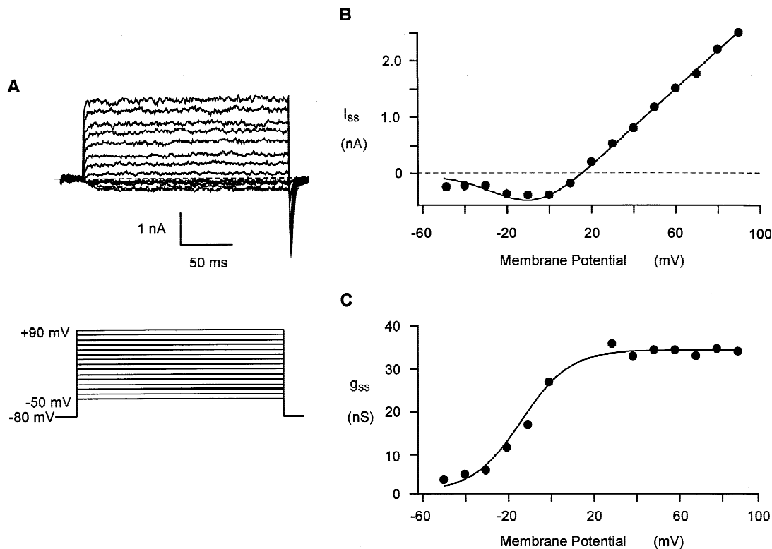
Fig. 4. Membrane currents in C1 cells with 10 \mu\text{M} [\text{Ca}^{2+}]_i . (A) Currents were elicited by 200 ms voltage steps from -50 to +90 mV in 10 mV increments from a holding potential of -80 mV in \text{K}^+ solution. Time between pulses was 5 s. (B) Steady-state current-voltage relationship for the experiment shown in A. Steady-state current ( I_{ss} ) was determined as the plateau current measured between 10 and 190 ms after the beginning of the depolarizing voltage step. A current-voltage fit indicated a reversal potential of \sim 15 mV and a V of \sim -13 mV and k = 11.5 mV. (C) Steady-state conductance-voltage relationship from the experiment shown in A. The steady-state conductance ( g_{ss} ) was calculated from (B) and plotted against the depolarizing step potential. A Boltzmann curve was fitted to the data with V_{1/2} of -13.1 mV and k = 11.5 mV.
