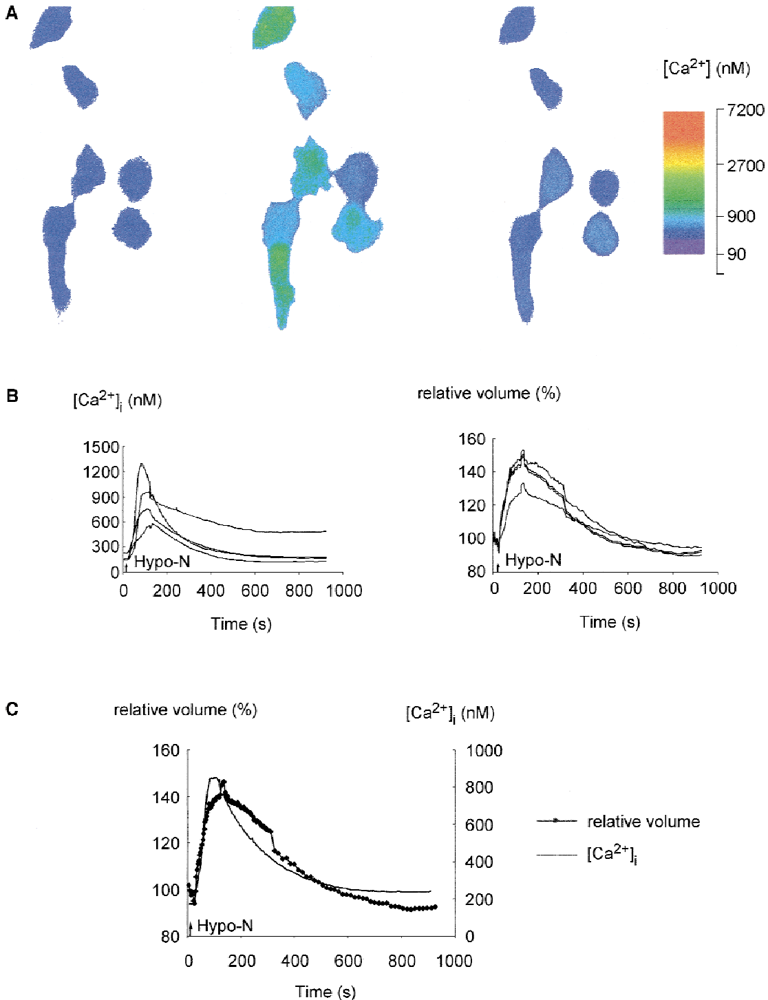
Fig. 1. Changes in [Ca^{2+}]_i and cell volume in C1 cells in response to a hypotonic (50% Na^+ solution with 4 mM CaCl_2 ) external solution. (A) Shown are pseudo color representations of fura-2 ratio images. Images were obtained in normal Na^+ solution (left), 80 s (middle) and 780 s (right) after the change to the hypotonic Na^+ solution. (B) Time course of changes in [Ca^{2+}]_i (left) and cell volume (right) in C1 cells shown in (A) after application of a hypotonic external solution (Hypo-N). (C) Time course of averaged changes in [Ca^{2+}]_i and relative volume of the cells shown in (A). The arrows in (B) and (C), respectively, mark the beginning of the solution change.
